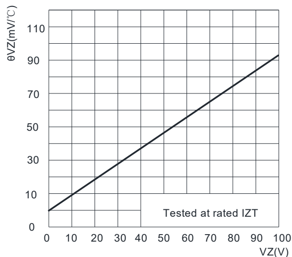
FIG2: Typical Temperature Coefficients
